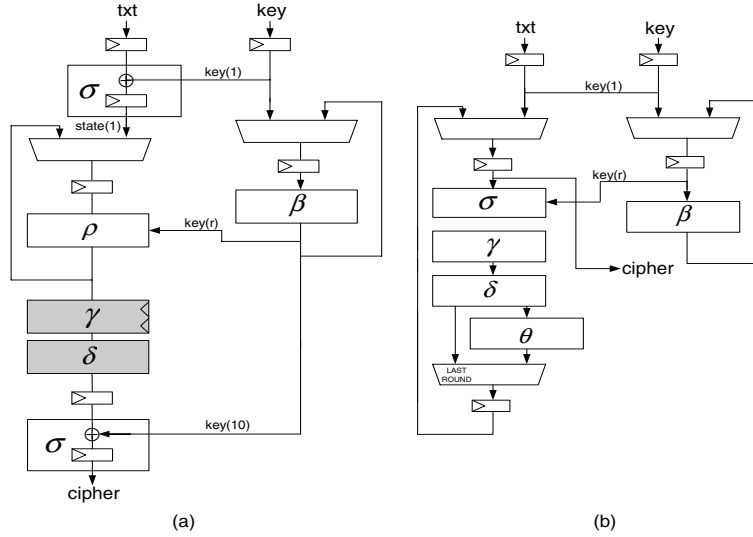
Fig. 7. AES Rijndael: loop architecture (a) and (b).
