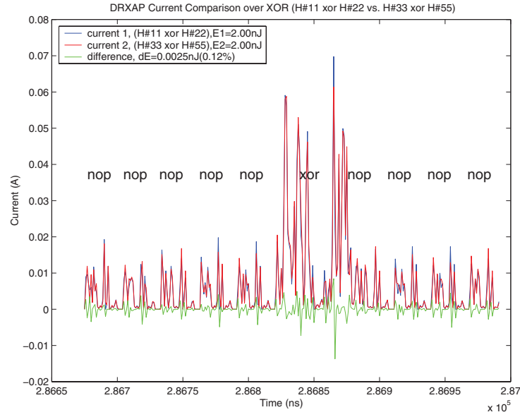
Fig. 8. Power Simulation. Secure XAP executing XOR
