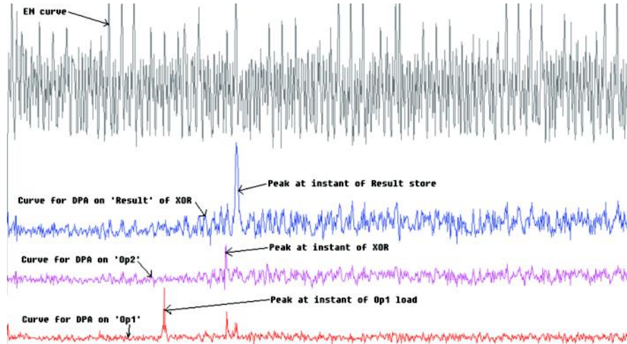
Fig. 3. DEMA Results
