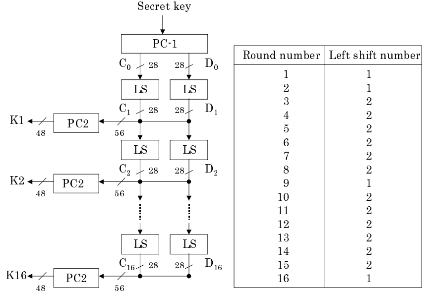
Fig. 3. Key Schedule
