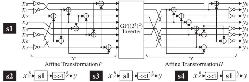
Fig. 2. Camellia S-Boxes
