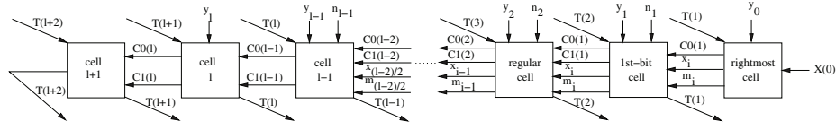
Fig. 6. Schematic view of the complete systolic array
